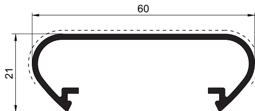
PLC 143
